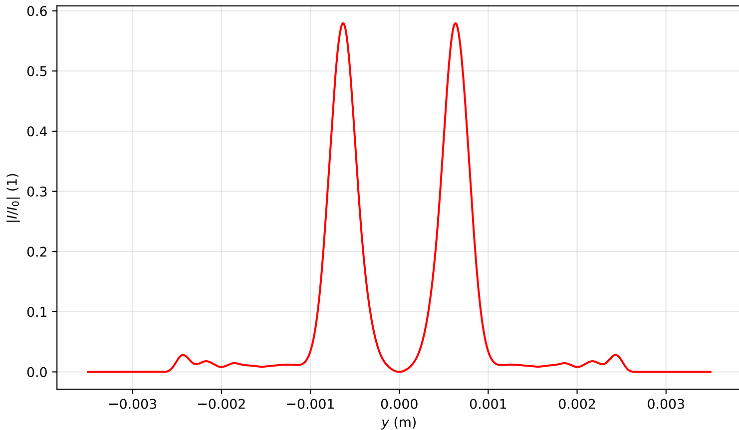
Intensity profile I(x=0, y, z=2.149)/I_0 , \text{Pin}=7.0\text{Pcr} , artificial time
